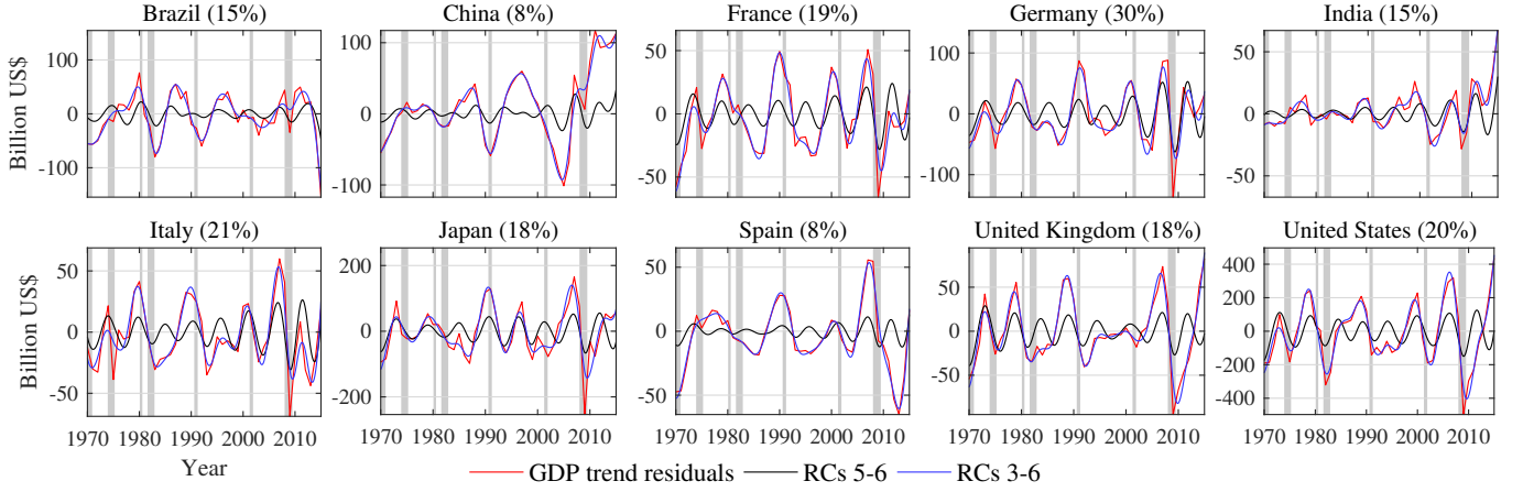
Figure 8. Same as Fig. 7 but for a reconstruction with RCs 5-6 (black), as well as the sum of RCs 3-4 and RCs 5-6 (blue). The second RC pair captures 18% of the trend residuals' total variance, while the variance it captures in the GDP of each country is given in the legend of each panel (in %).
