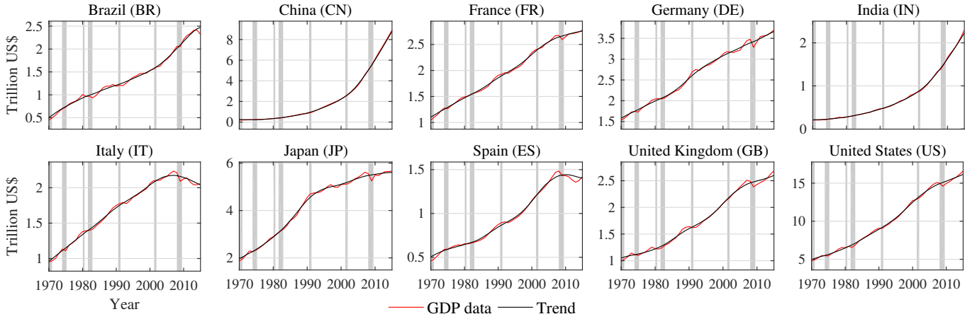
Figure 6. Annual GDP data of ten major economies from 1970 to 2015 (red) and estimated trend component (black) captured by RCs 1-2 from a complementary M-SSA analysis of the WDI dataset. The window length is M = 12 years and all 12 EOFs are varimax rotated. The vertical bars in all panels indicate NBER-defined US recessions. The trend component captures 99% of the total variance. Note the different scales on the y -axis.
