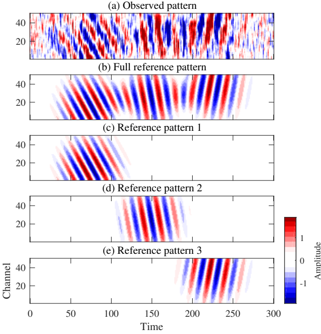
Figure 1. Spatio-temporal oscillations in the presence of strong correlated noise. (a) Observed pattern; and (b) noise-free reference pattern with D = 50 channels of length N = 300 . The reference pattern is composed of three different spatio-temporal oscillations in panels (c–e), with the oscillation period T = 20 in all three patterns. Superimposed on the reference signal is spatio-temporally correlated noise, with the signal-to-noise ratio set to 1.5.
