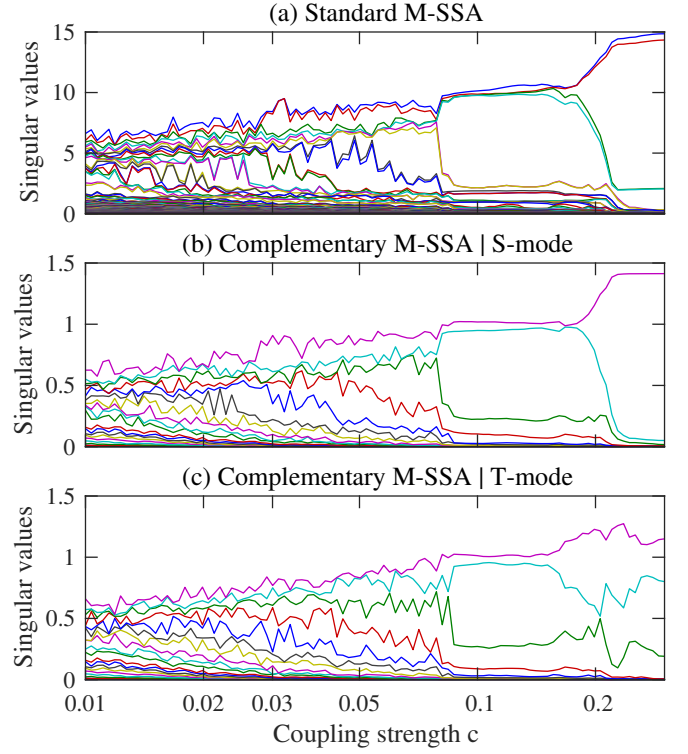
Figure 3. Synchronization for a chain of J = 20 coupled Lotka-Volterra oscillators (15). Spectrum of singular values from (a) the standard M-SSA algorithm, and (b,c) from the complementary M-SSA algorithm, with a subsequent complex-EOF analysis of ST-EOFs 1-2; here the latter analysis uses (b) the S-mode, and (c) the T-mode. The M-SSA window length is M = 30 and the 20 leading EOFs are varimax rotated.
