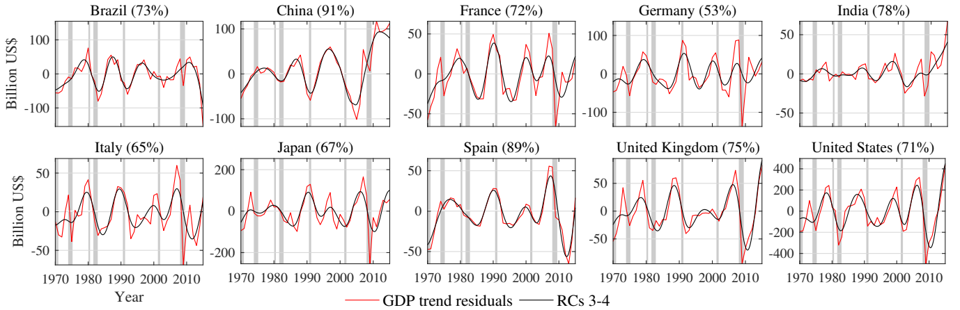
Figure 7. GDP trend residuals (red) and reconstruction with RCs 3-4 (black) from the M-SSA analysis in Fig. 6. This RC pair captures 73% of the trend residuals' total variance, while the variance it captures in the GDP of each country is given in the legend of the corresponding panel (in %). Note the different scales on the y -axis.
