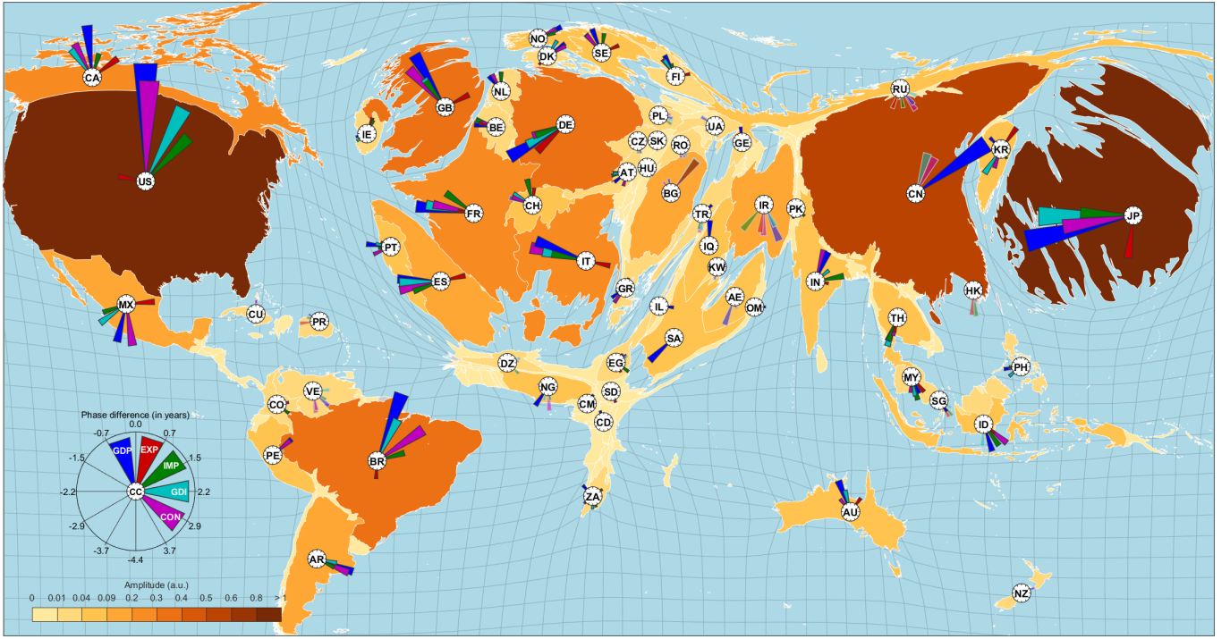
Figure 12. Same as Fig. 11, but for complex S-EOF 2.
