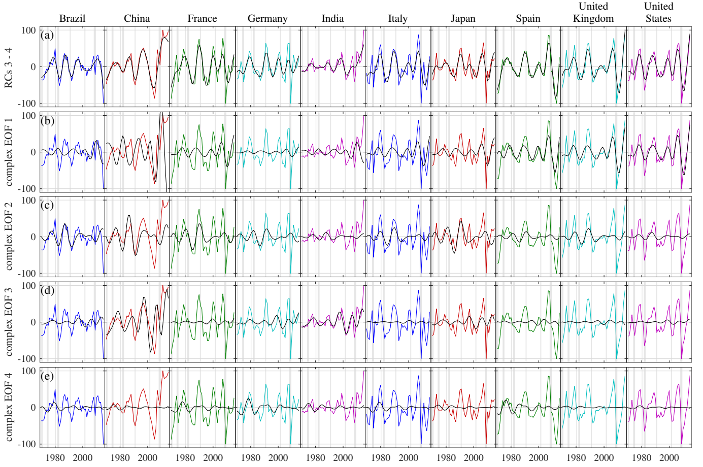
Figure 10. GDP trend residuals of ten major economies (in color) and their reconstructions (black) with (a) RCs 3-4, as reproduced from Fig. 7; and (b-e) partial RCs 1-4 from the complex EOF analysis in Fig. 9. For ease of comparison, the GDP trend residuals have been rescaled to the interval [-100, 100] .
