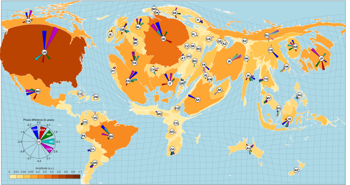
Figure 14. Same as Fig. 11, but for complex S-EOF 4.
