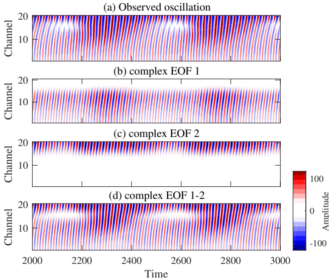
Figure 4. Chain of purely periodic oscillators (15) at coupling strength c = 0.1 . (a) Observed spatio-temporal oscillation of the x -components; and (b-d) partial RCs from a complex EOF analysis in S-mode. Parameter values and details given in Fig. 3.
