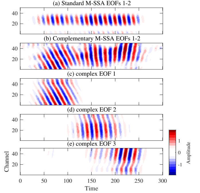
Figure 2. Reconstruction of spatio-temporal oscillations with the leading oscillatory pair RCs 1-2 of (a) the standard M-SSA algorithm and (b) the complementary M-SSA algorithm. The window length M = 30 and the leading 10 EOFs varimax rotated. Panels (c–e) show partial RCs from a reconstruction with the three leading EOFs of a subsequent complex EOF analysis of M-SSA EOFs 1-2 of panel (b). The complex EOF analysis in T-mode, with the 10 leading complex T-EOFs varimax rotated.
