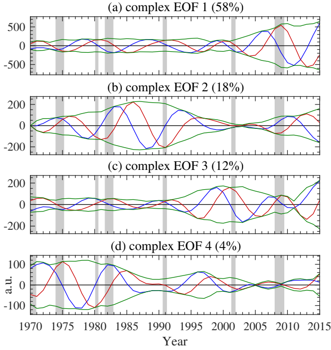
Figure 9. Complex EOF analysis in T-mode of ST-EOFs 3-4 that corresponds to RCs 3-4 in Fig. 7. Shown are the complex-valued temporal patterns that characterize the spatio-temporal oscillations in the partial RCs, based on a reconstruction with the four leading complex EOFs. The real and imaginary parts are plotted in blue and red, respectively, while the envelope is plotted in green. The variance captured by each mode is given in the legend of each panel (in %).
