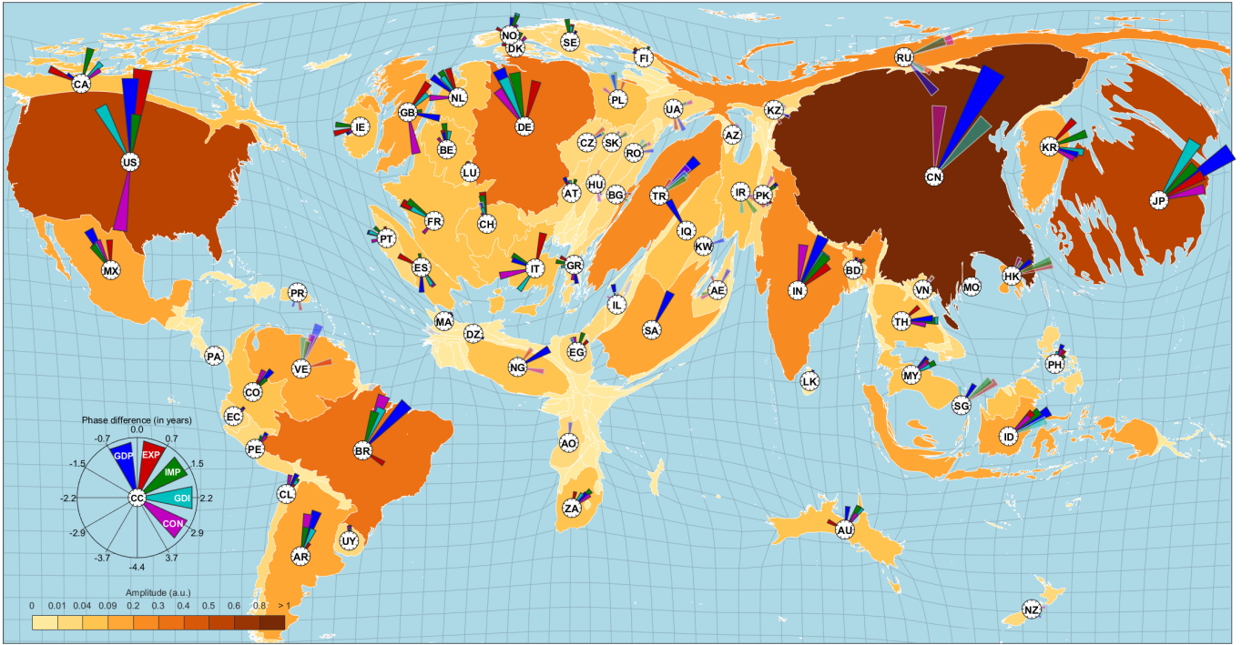
Figure 13. Same as Fig. 11, but for complex S-EOF 3.
