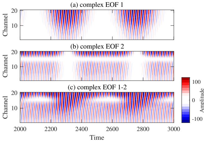
Figure 5. Same as Fig. 4, but with partial RCs from a complex EOF analysis in T-mode.
